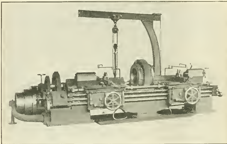
LODGE & SHIPLEY DOUBLE END AXLE LATHE.
